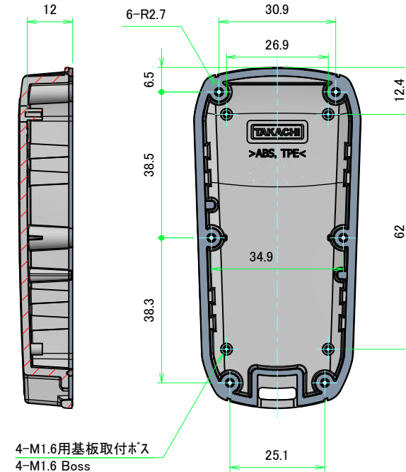
E-E (1:1)
