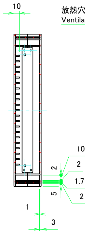
B-B (1:4)
