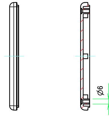
C-C (1:2.5)
