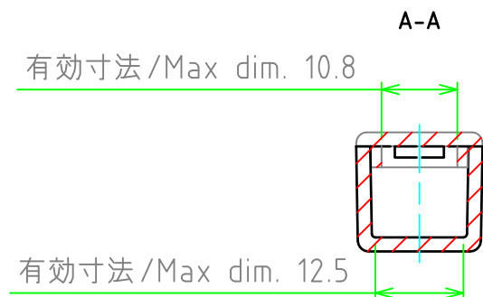
下蓋 (内視) Cover (Internal View)
