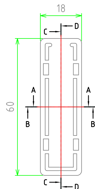
下蓋 (内視) Cover (Internal View)
