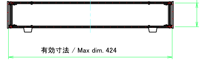
C-C (1:5)
