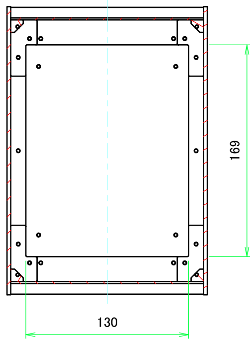
B-B (1:3)
