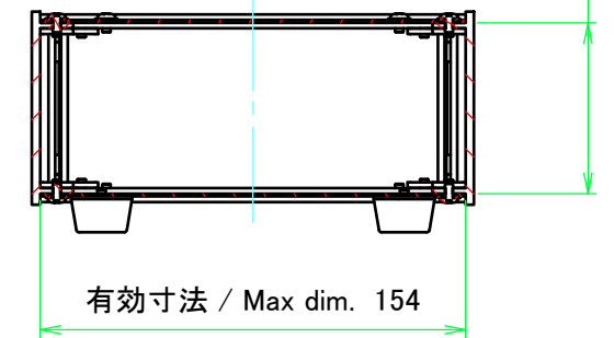
C-C (1:3)
