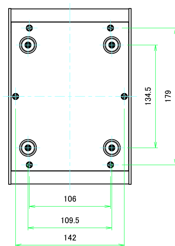
F view
