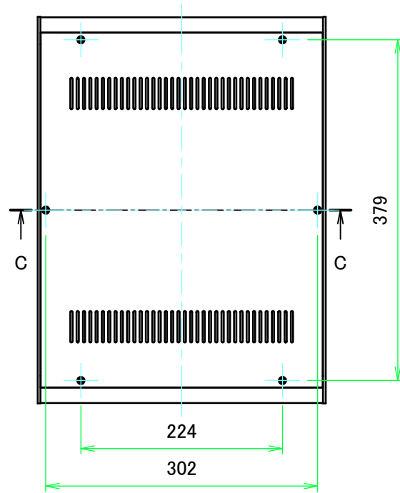
E view
