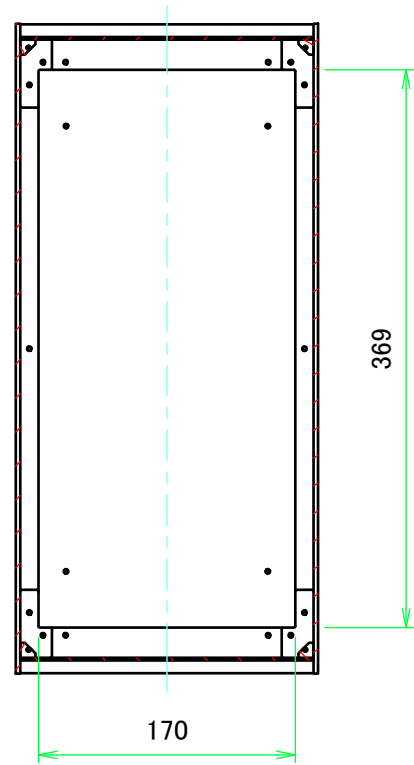
B-B (1:5)
