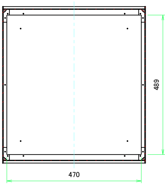
B-B (1:7)
