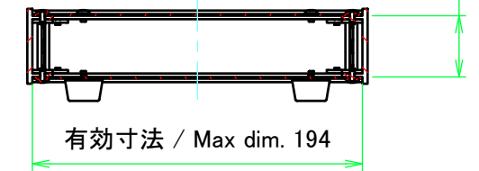
C-C (1:4)
