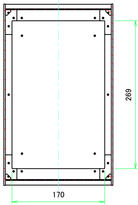
B-B (1:4)
