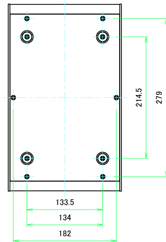
F view
