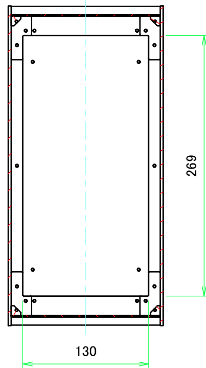
B-B (1:4)
