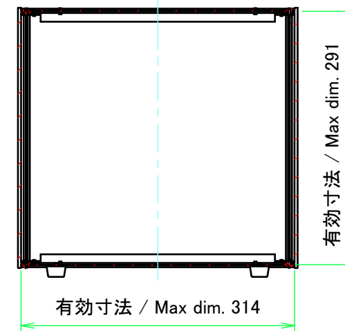
C-C (1:6)
