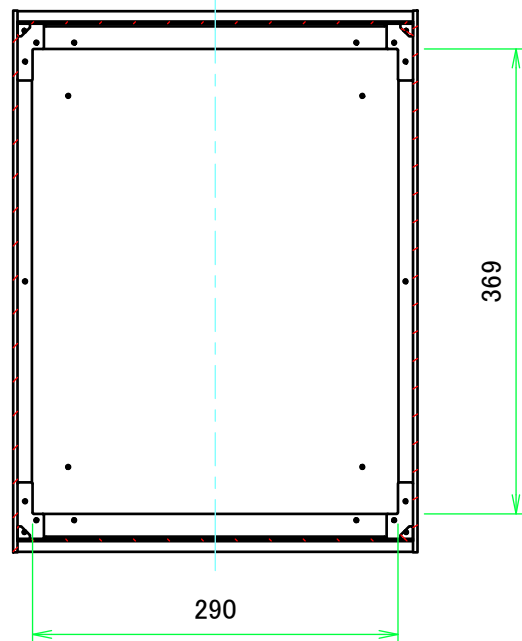
B-B (1:6)
