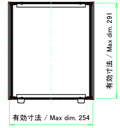
C-C (1:6)
