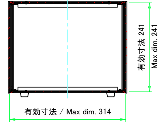
C-C (1:6)
