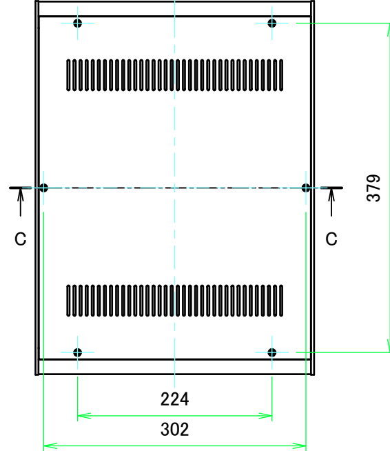
A view
