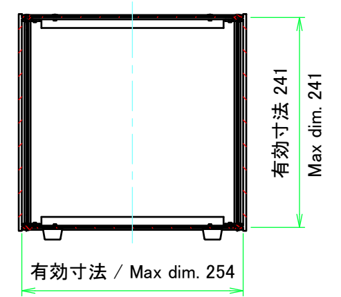
C-C (1:6)
