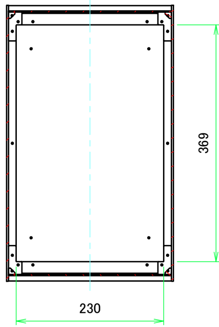
B-B (1:6)
