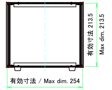
C-C (1:6)
