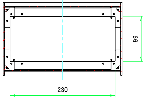
B-B (1:4)
