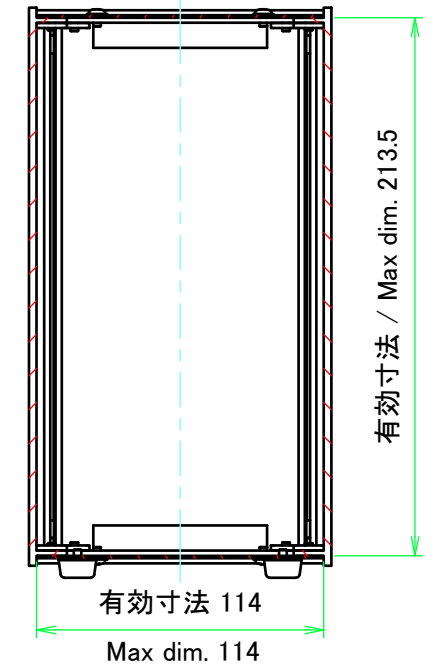
C-C (1:3)
