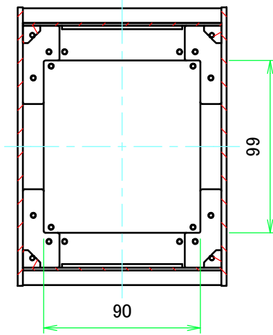
B-B (1:3)
