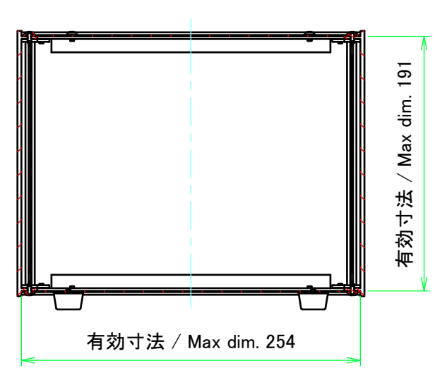
C-C (1:4)
