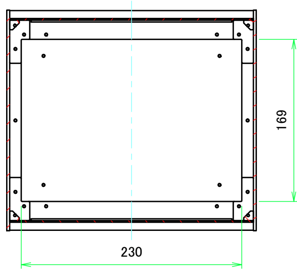
B-B (1:4)
