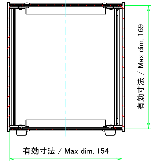
C-C (1:3)
