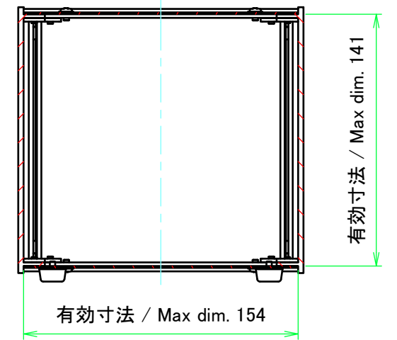
C-C (1:3)
