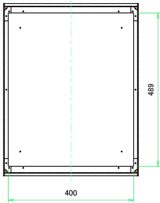
B-B (1:7)
