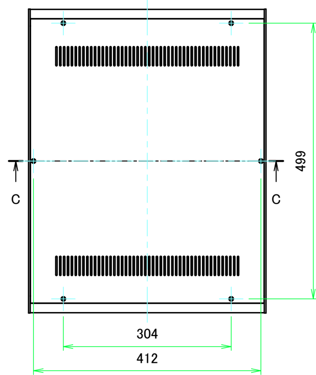
A view
