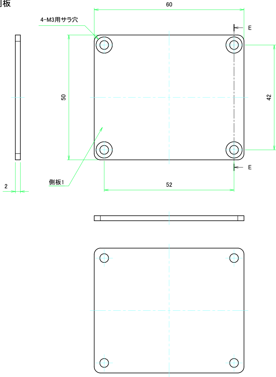
E-E (1.5:1)
