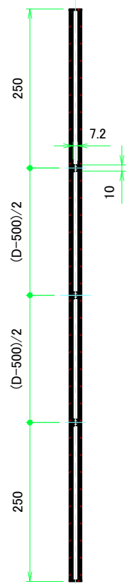
C-C (1:6)
