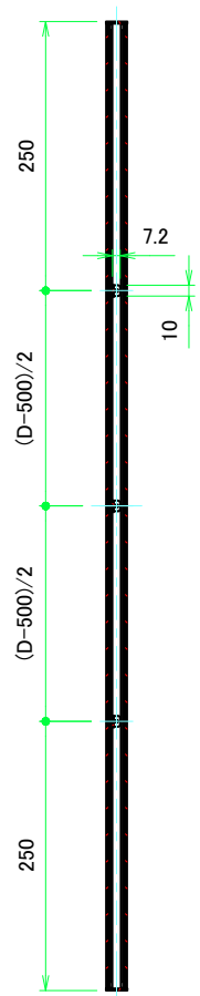
C-C (1:5.5)
