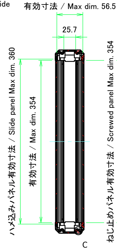
B-B (1:5)
