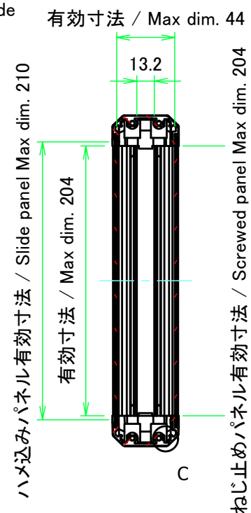
B-B (1:4)
