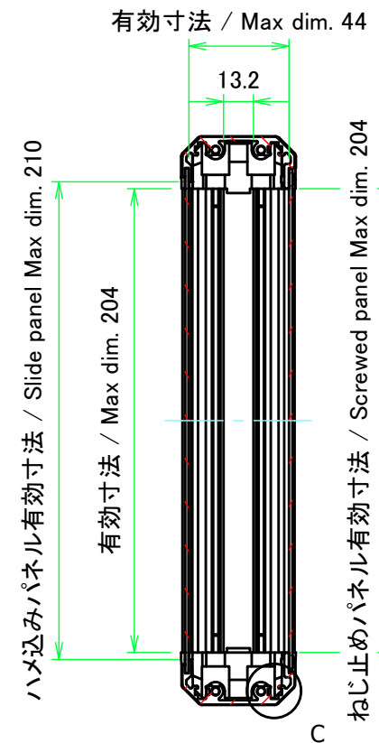
B-B (1:3)
