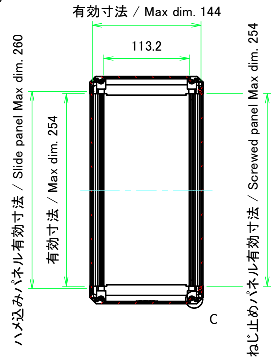
B-B (1:5)
