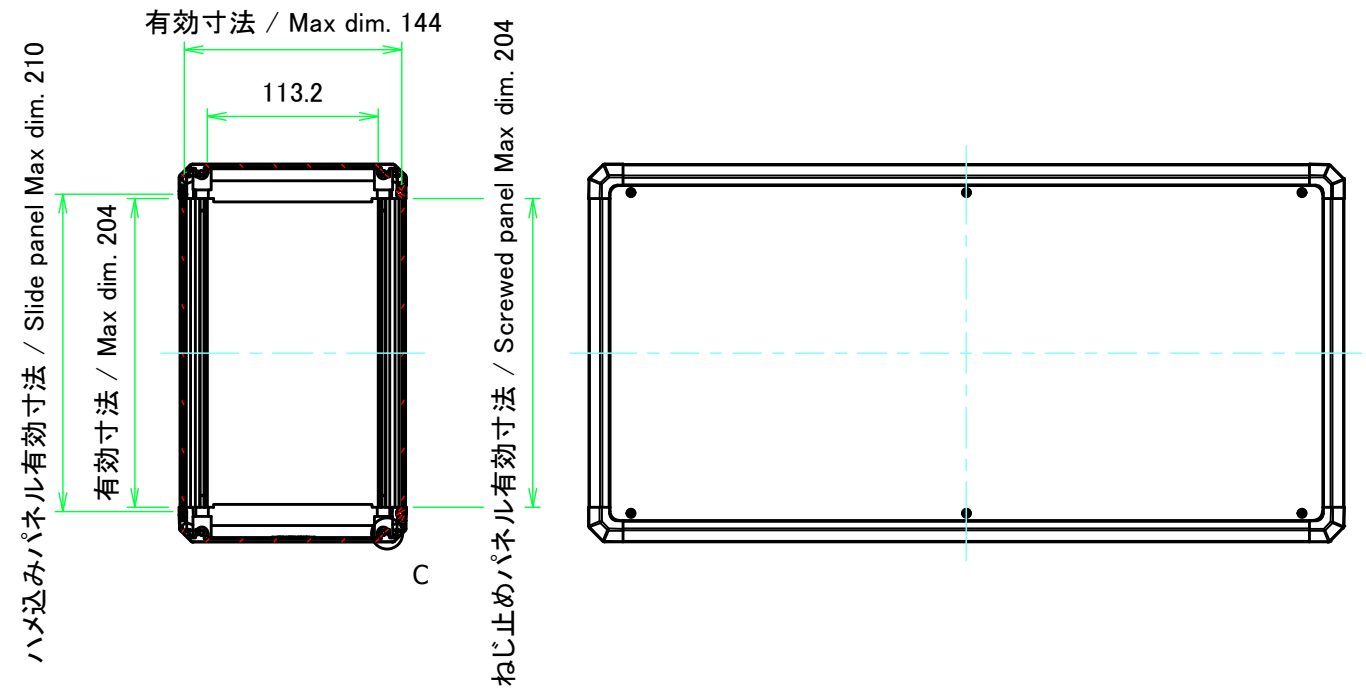
B-B (1:5)
