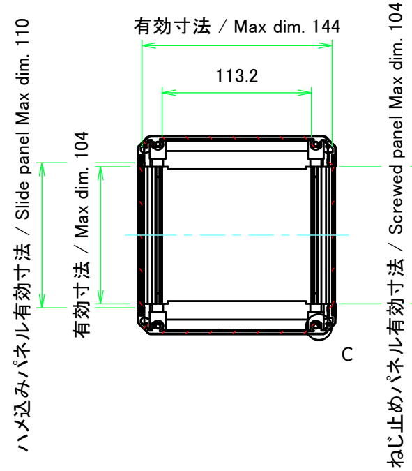
B-B (1:4)
