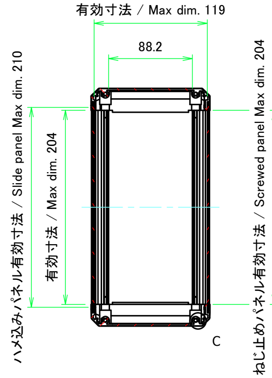
B-B (1:4)
