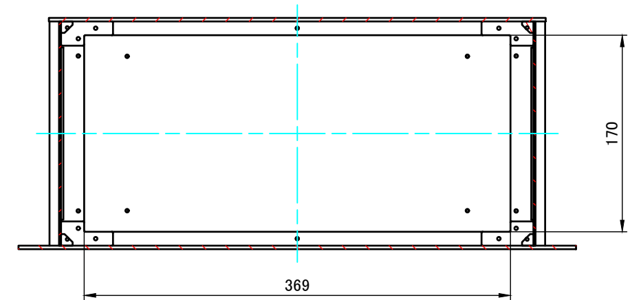
B-B (1:4.5)
