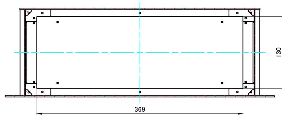
B-B (1:4)
