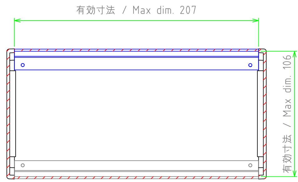
ネジ止めパネル(内視) Screwed panel (Internal View)
